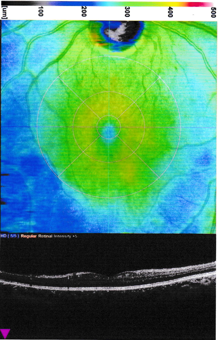
Normative Database
